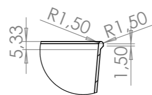
DETAIL B SCALE 2 : 5
